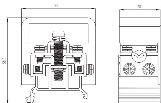
RMJ 2.5
