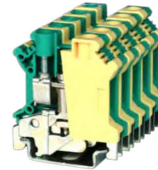
RTB 10-PE
