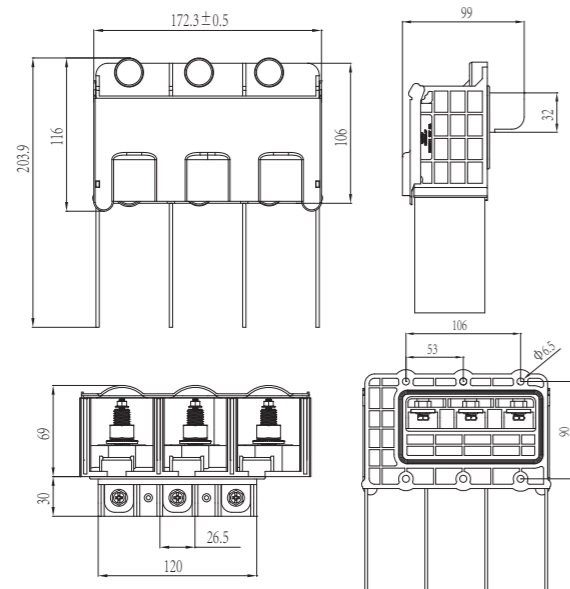
RBS300A-3P
